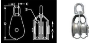
TWIN SWIVEL BLOCK 柔型双滑轮
