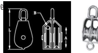
DOUBLE SWIVEL PULLEY WITH RING
