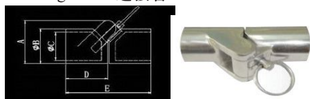
Swivelling Joints 连接管
