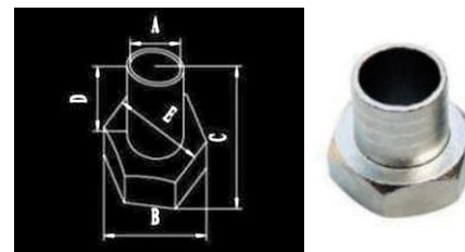
Connection 接头
