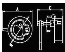
Turning Lock Lift Handle 地板锁
