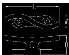
Aluminum cleat 铝索栓
