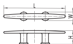
Cleat with threaded stud 螺纹索栓
