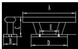
Oval Tube Cleat 椭圆管式索栓
