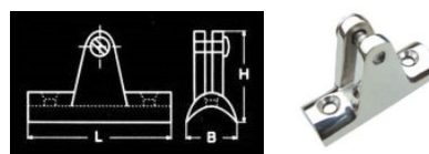
Deck Hinge with Concave 栓式山型座
