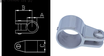
Tope Slide 滑套
