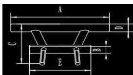
Round Tube Cleat 圆管式索栓
