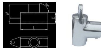
Tees with cable eyelet 90° 90度带缆孔三通
