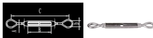
TURNBUCKLE DIN1480 Eye/Eye 开体花篮
