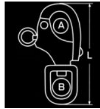
SWIVEL SNAP SHACLE WITH EYE 卸扣
