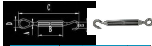
TURNBUCKLE,TYPE HOOK -EYE 开体花篮
