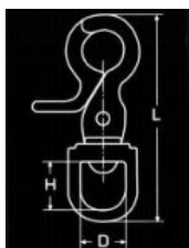
TRIGGER SNAP HOOK WITH SWIVEL EYE 挂钩
