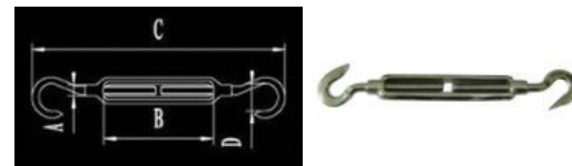
TURNBUCKLE,TYPE HOOK-HOOK 开体花篮
