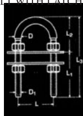
U BOLT WITH LATCH U 型栓
