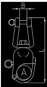
SWIVEL SNAP SHACLE WITH JAW 卸扣
